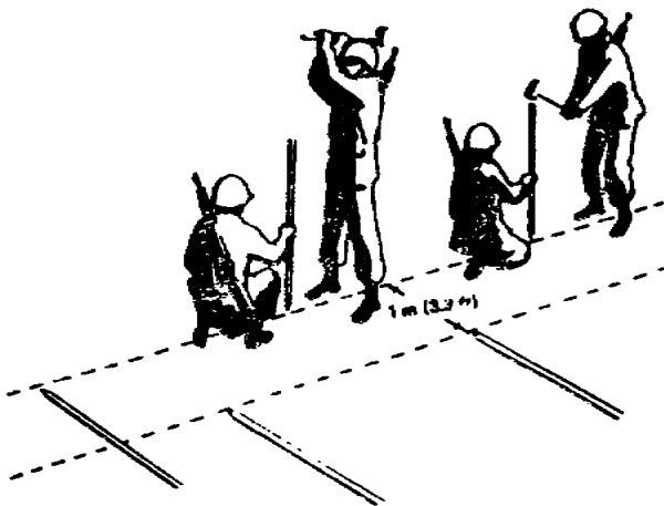
Figure 4-25. Installing front row pickets for triple concertina fence.
